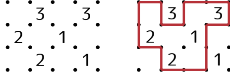
Fig. 3. Small example of Slitherlink challenge, and its solution.
