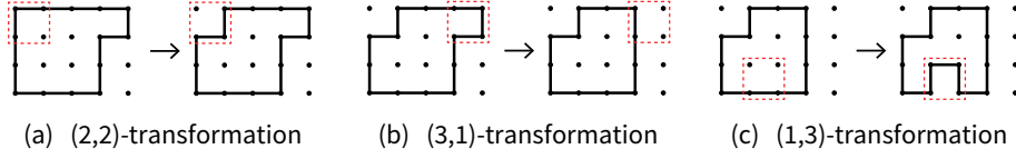
Fig. 2. Three transformations.
